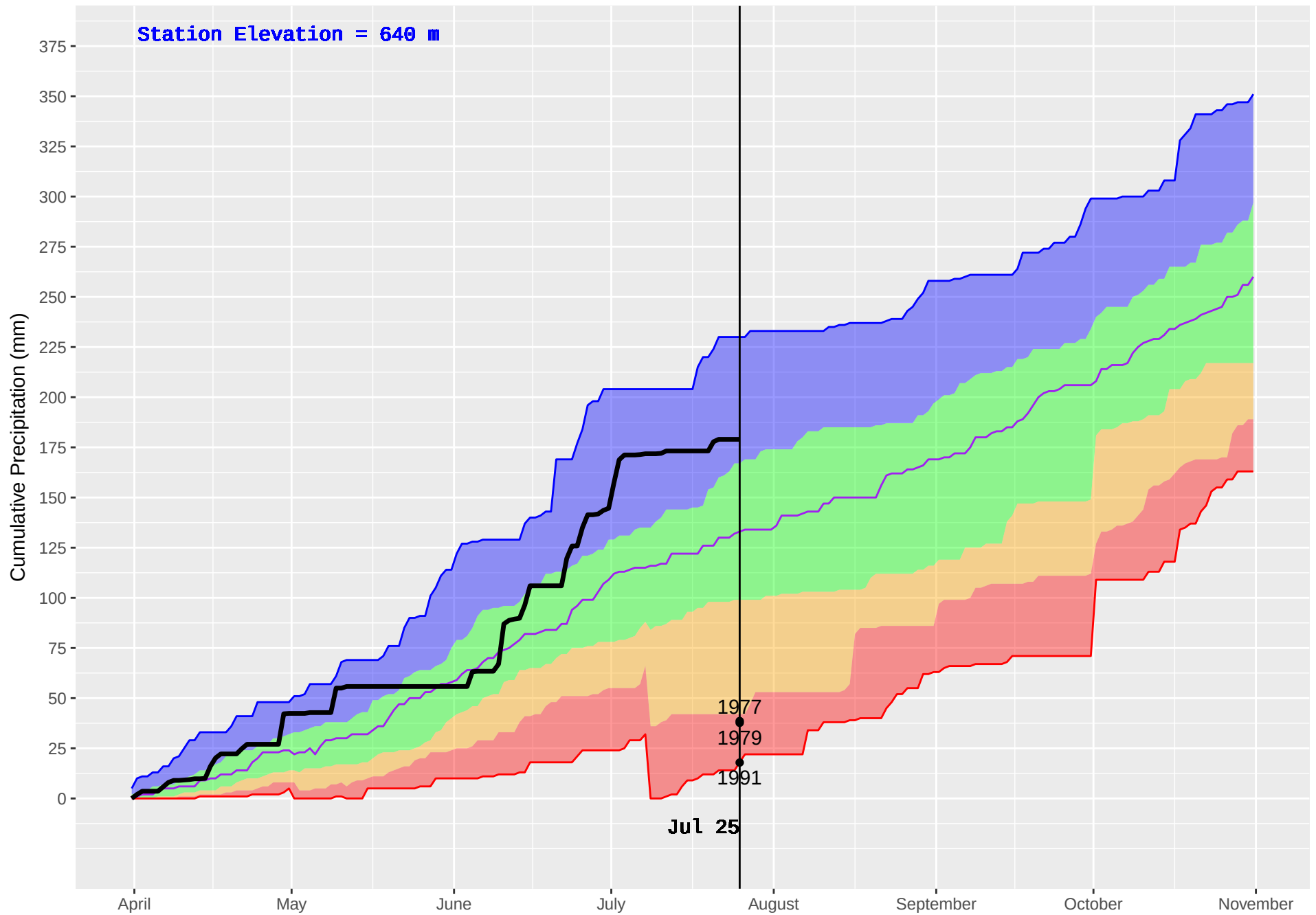
TURTLE (286) : Historical (1977–2016) and Current (2018) Noon Cumulative Precipitation
